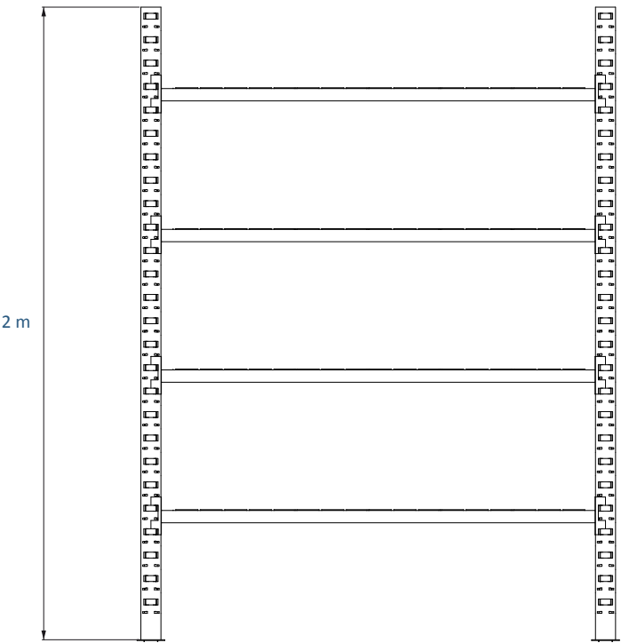
Vista Frontal
